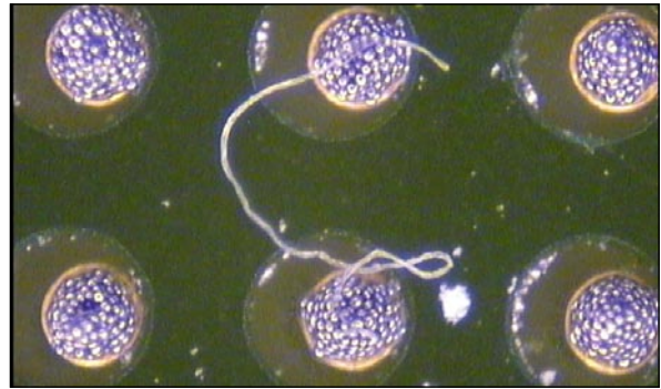
Figure 3 – BGA with fibre and dust
