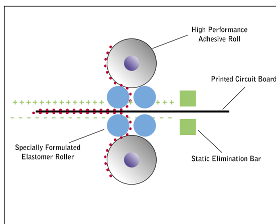
Figure 1 – The contact cleaning process
